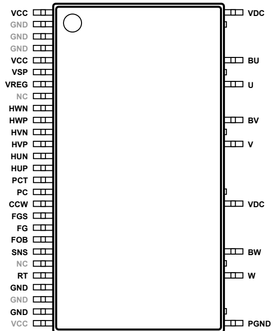
Figure 3. Pin Configuration
