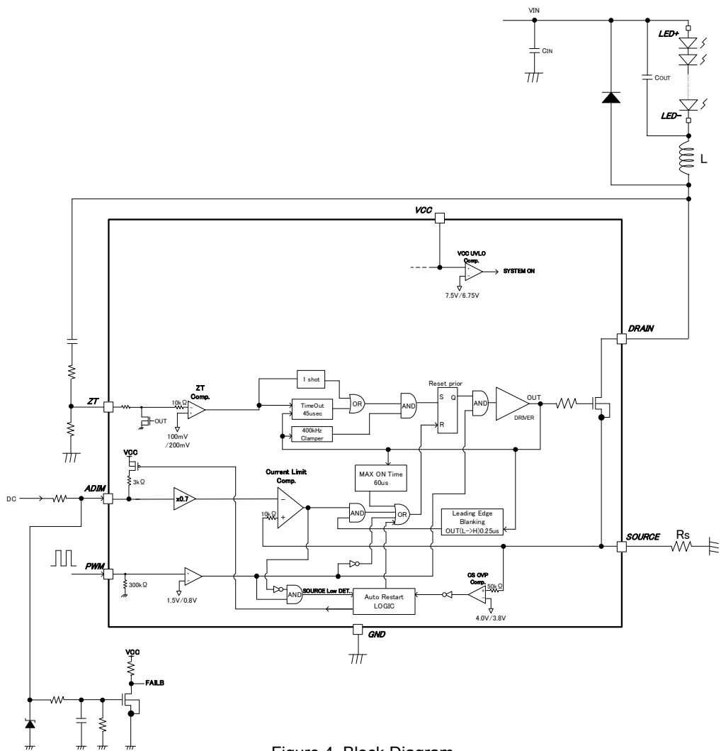
Figure 4. Block Diagram
