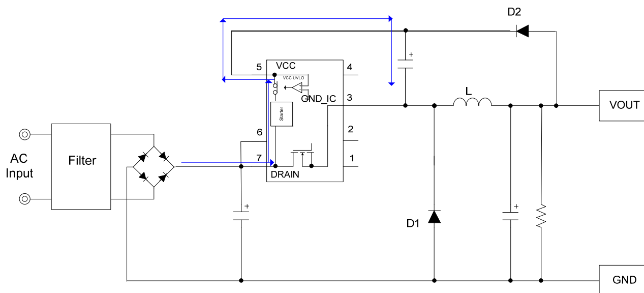
Figure 5. Start circuit
