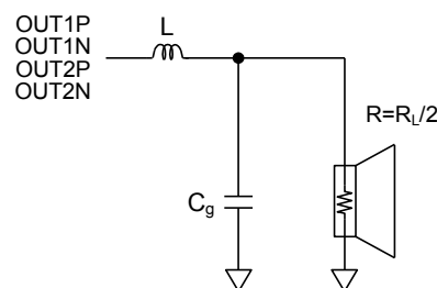
Figure 75. Output LC filter 2
