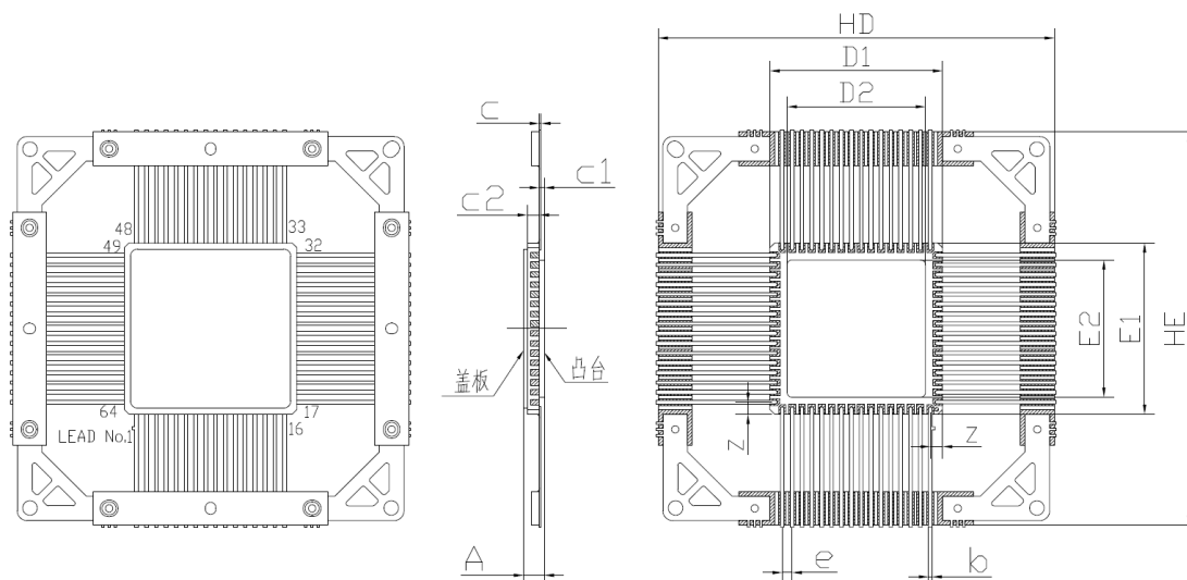
Figure 6. BM2711MQRH's Packaging(CQFP64)
