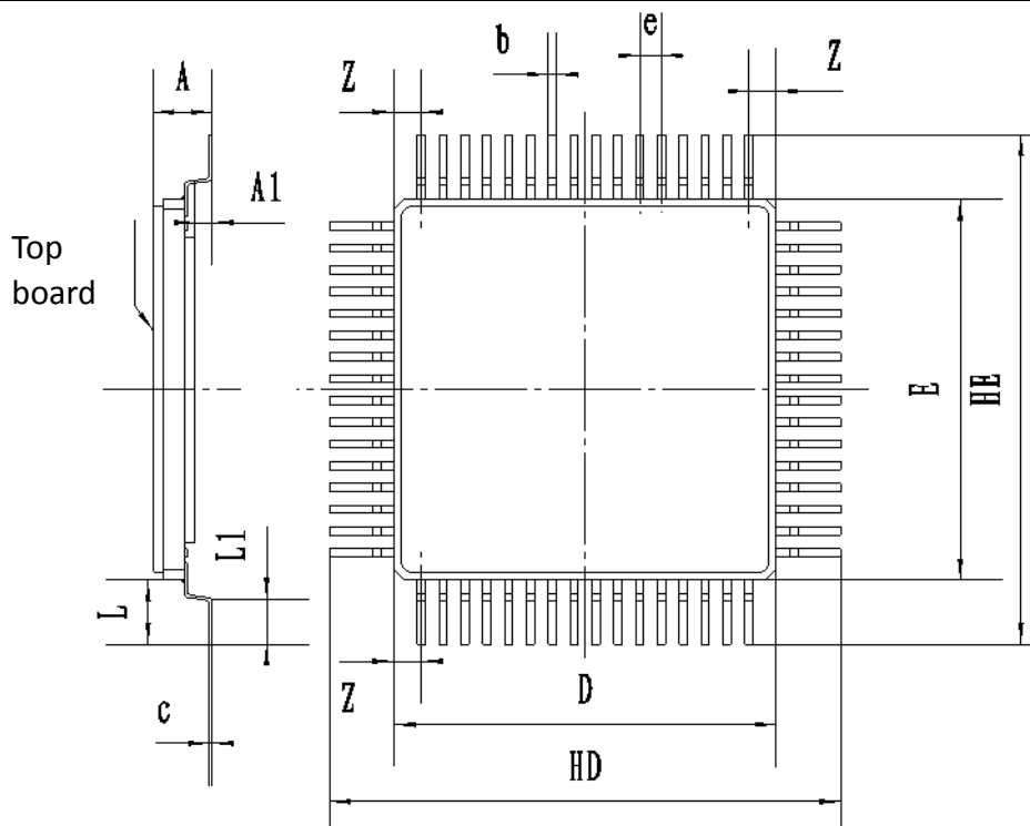
Figure 7. Cutting Forming Diagram
