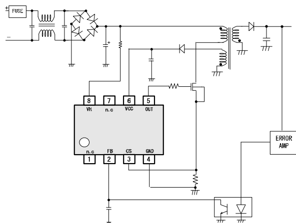
Figure 1. Application Circuit
