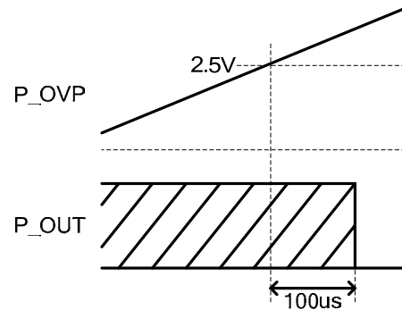
Figure 30. Timing Chart
