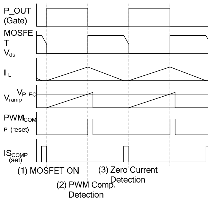
Figure 25. The Switching Timing Chart.
