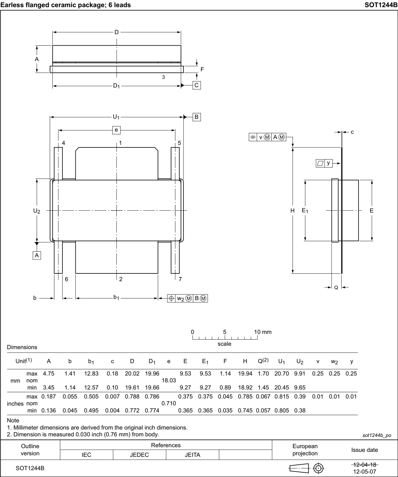
Fig 10. Package outline SOT1244B
