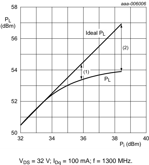
Fig 4. Output power as a function of input power; typical values
