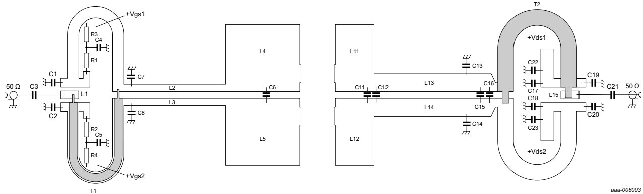
Fig 1. Schematic for class-AB production test circuit
