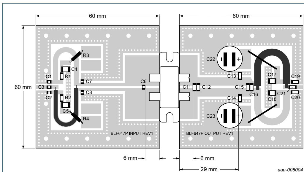
Fig 2. Component layout for class-AB production test circuit
