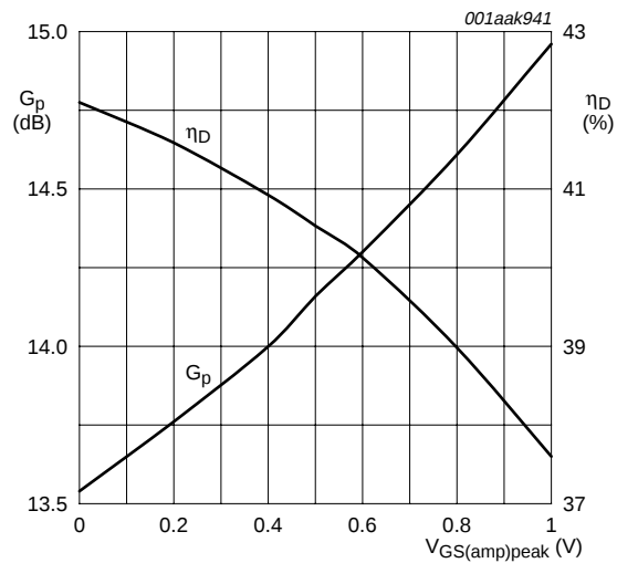
Fig 10. Power gain and drain efficiency as function of peak amplifier gate-source voltage; typical values
