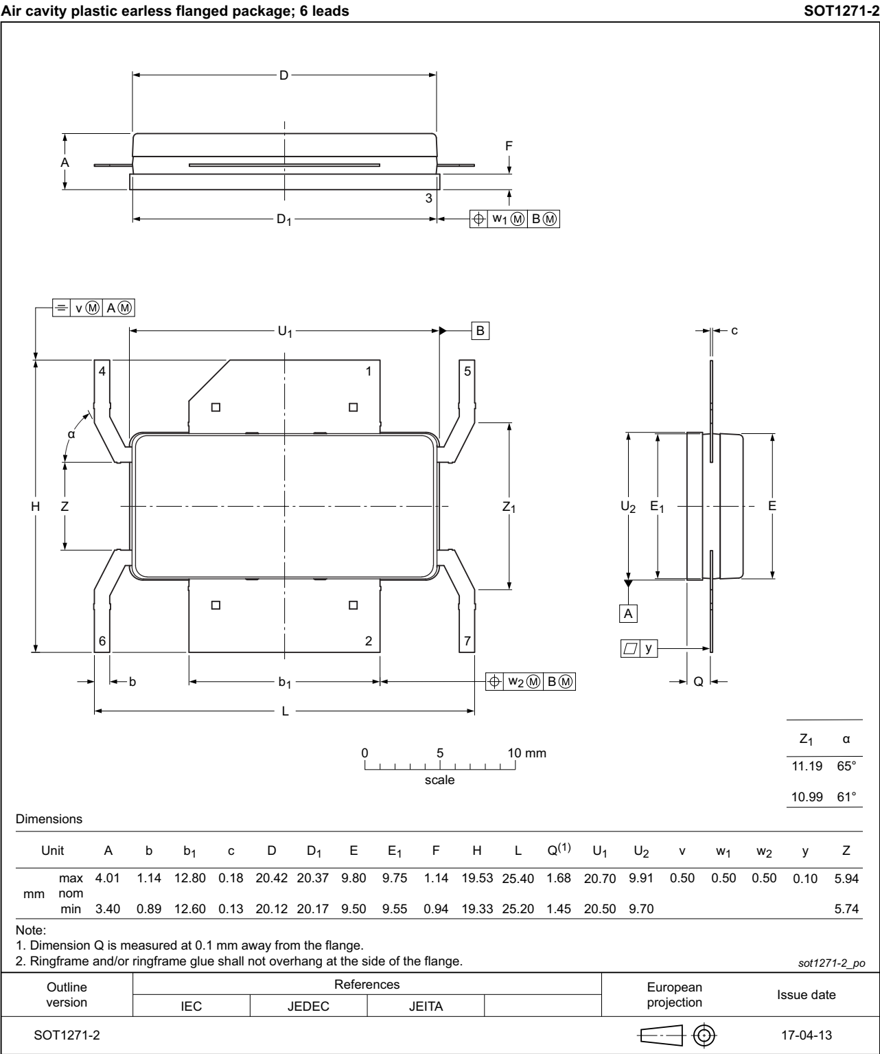
Fig 19. Package outline SOT1271-2
