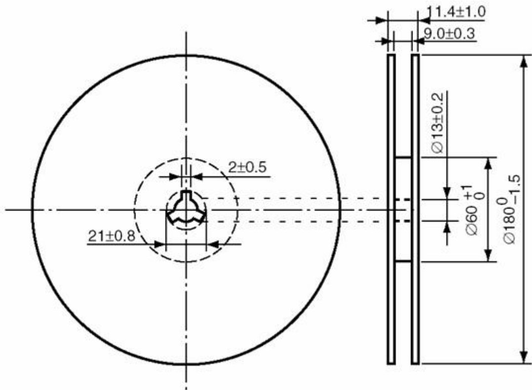
Reel dimension
