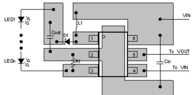
Figure 4. Recommended Component Placement
