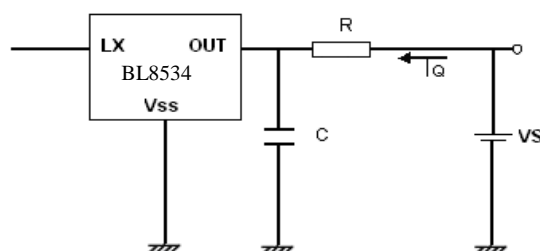
Figure 4: Quiescent current test circuit ( V_S=V_{out\_rt} \times 1.05 , R=1K\Omega , C=0.1\mu F )
