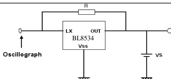
Figure 5: Oscillator frequency and duty cycle test circuit ( V_S=V_{out\_rt} \times 0.95 , R=1K\Omega )
