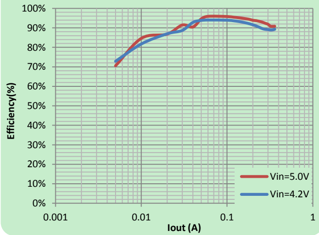
Efficiency Vout=12V
