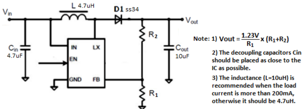
Figure1. BL8041 Typical Application Circuit
