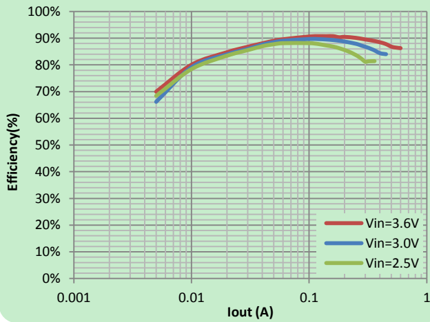
Efficiency Vout=5V
