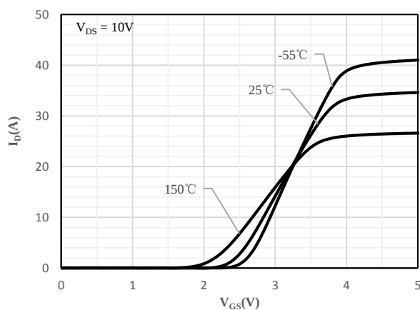
Fig 8 Transfer Characteristics
