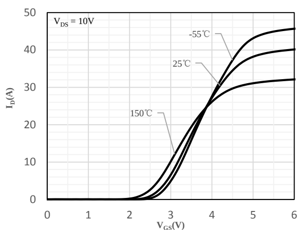
Fig 8 Transfer Characteristics
