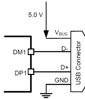
Fig 4. 12-w USB Charge Application
