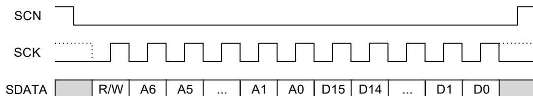
Figure 2-5 Three-Wire Interface Timing
