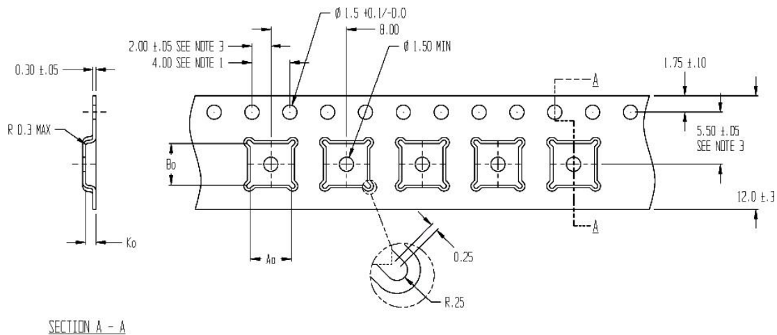
Figure 7-1 Tape Dimensions
