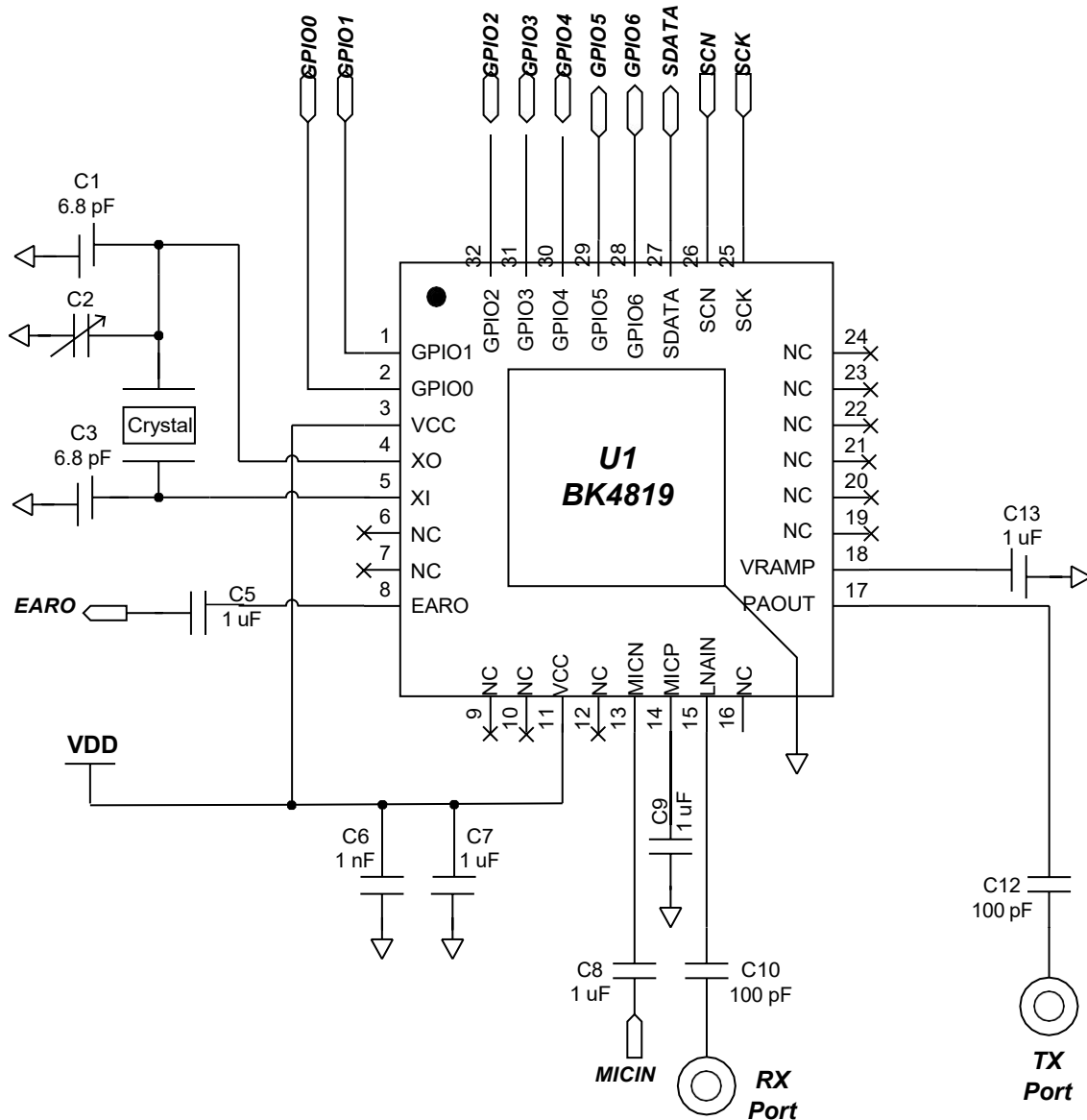
Figure 5-1 BK4819N Schematic
