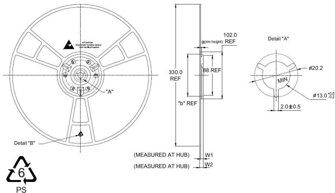
Figure 7-3 Reel Dimensions
