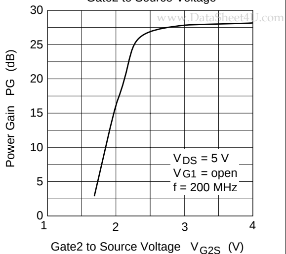
Power Gain vs. Gate2 to Source Voltage
