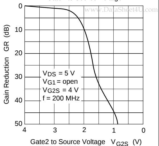
Gain Reduction vs. Gate2 to Source Voltage
