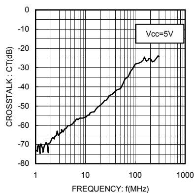
Fig.11 interchannel crosstalk
