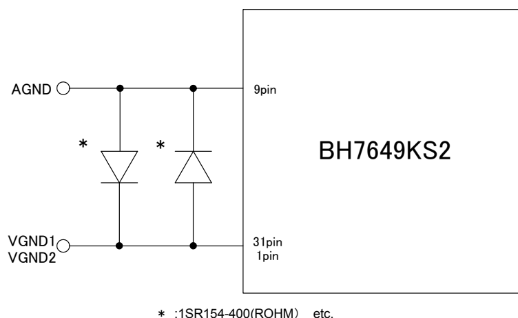
Fig.7 External diodes
