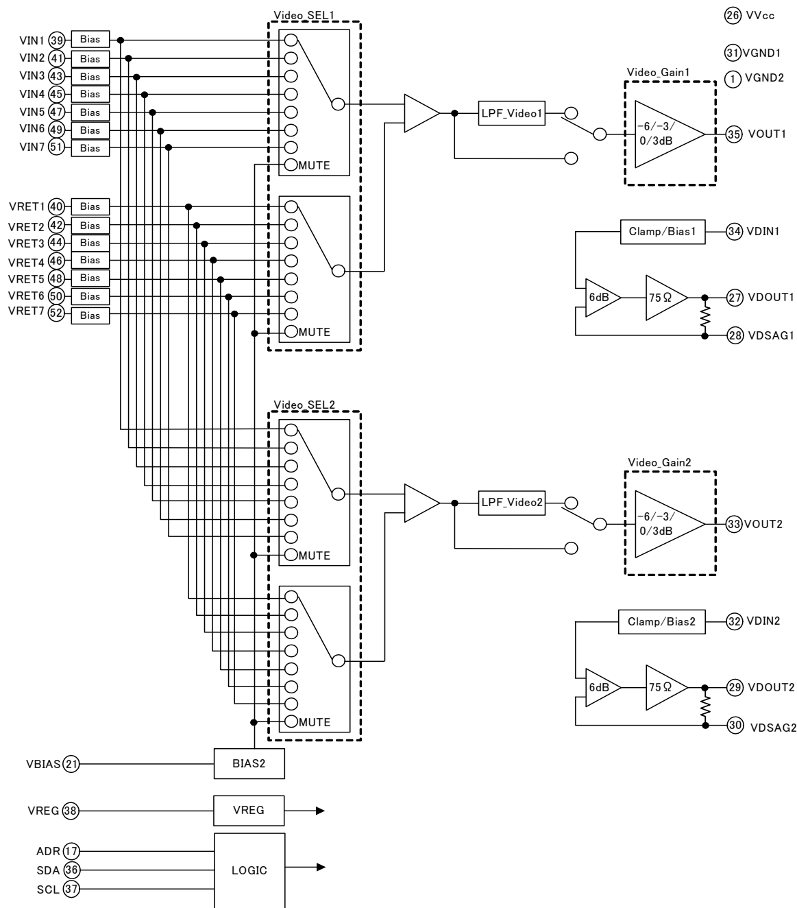
Fig.2 Block Diagram
