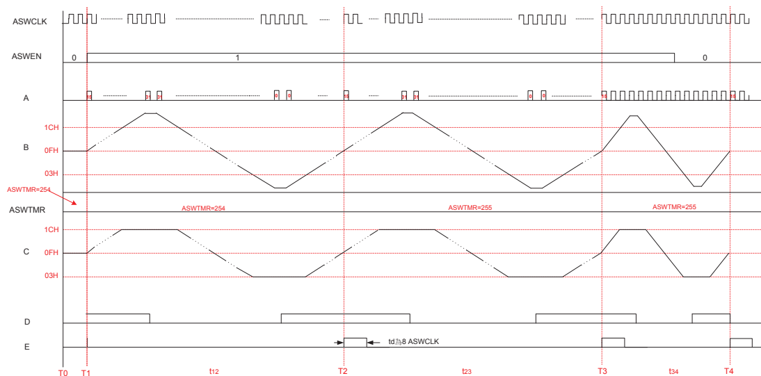
Sine Wave Generation Timing
