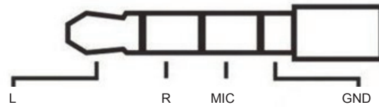
Non-international Standard 4-conductor Contact Pin Structure
