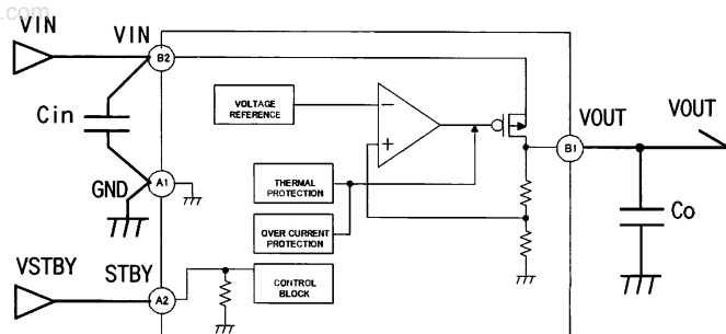
Fig.1 Block Diagram and Application Circuit
