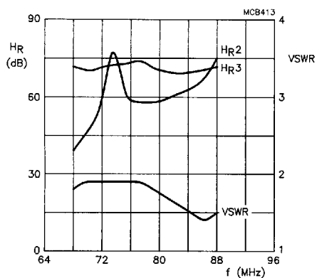
Fig.9 Second and third harmonic rejection as a function of frequency; P_L = 29 W; V_{S1} = V_{S2} = 12.5 V; typical values.
