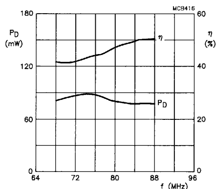
Fig.8 Efficiency and drive power as functions of frequency; P_L = 29 \text{ W} ; V_{S1} = V_{S2} = 12.5 \text{ V} ; typical values.
