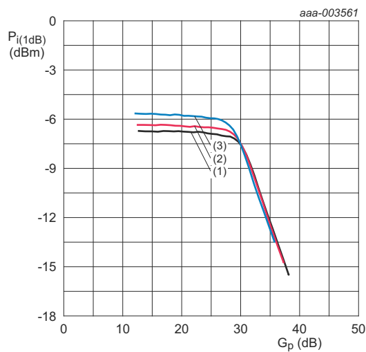
GS1 = LOW; GS2 = HIGH; V_{CC1} = 5\text{ V} ; V_{CC2} = 5\text{ V} ; f = 1950\text{ MHz} . (1) T_{amb} = -10^\circ\text{C} (2) T_{amb} = +25^\circ\text{C} (3) T_{amb} = +85^\circ\text{C}
