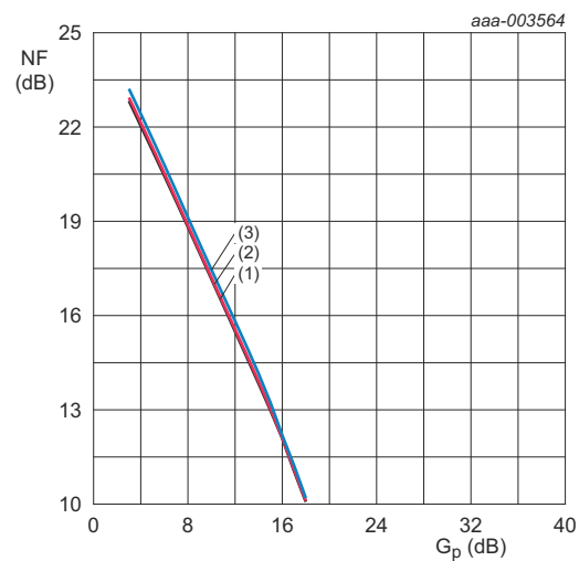
GS1 = HIGH; GS2 = LOW; V_{CC1} = 5\text{ V} ; V_{CC2} = 5\text{ V} ; f = 1950\text{ MHz} . (1) T_{amb} = -10^\circ\text{C} (2) T_{amb} = +25^\circ\text{C} (3) T_{amb} = +85^\circ\text{C}
