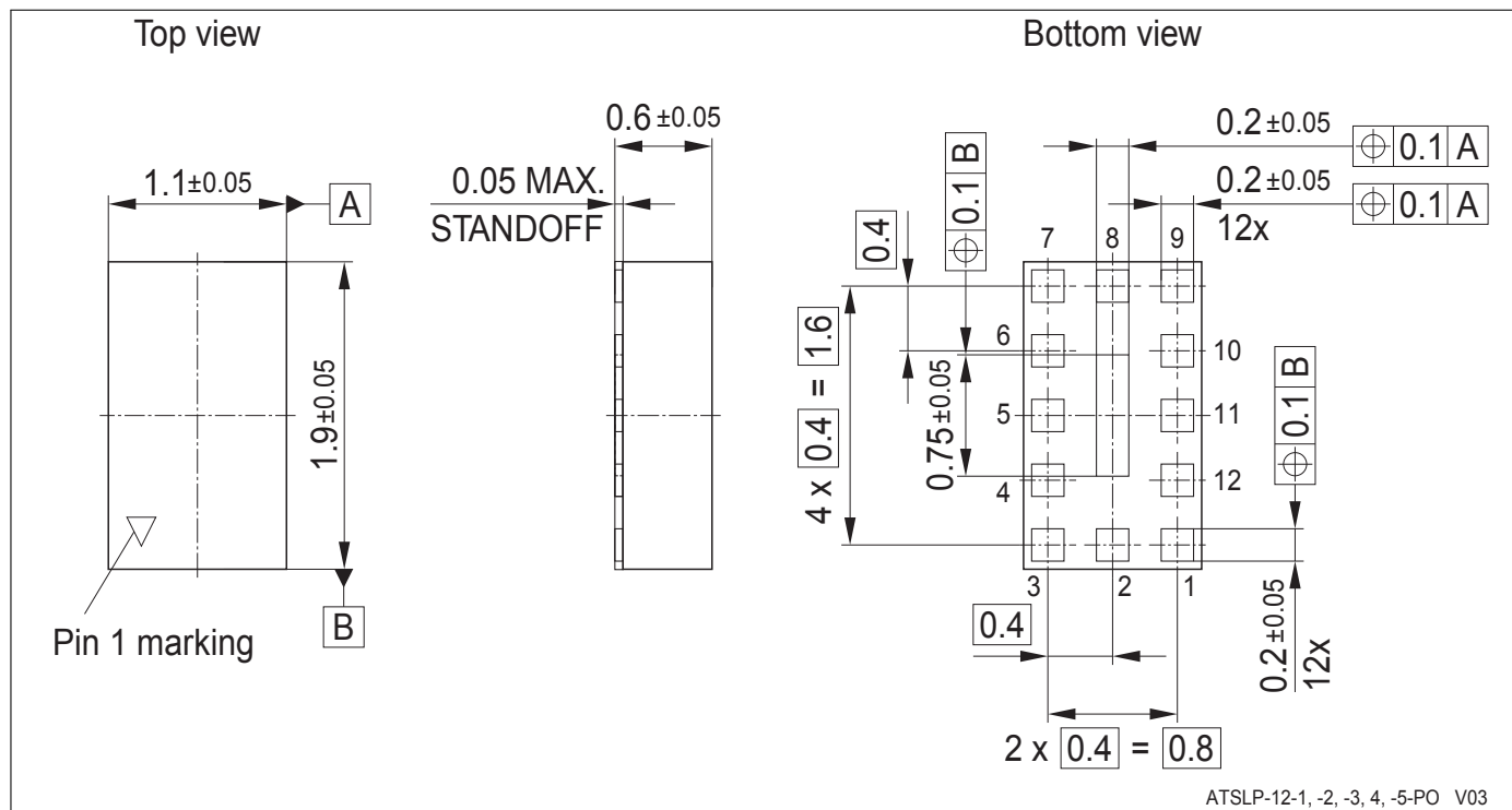
Figure 9: ATSLP-12-3 Package Outline (top, side and bottom views)
