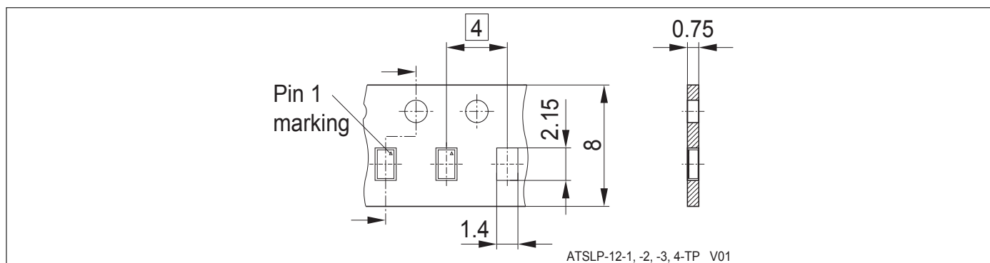
Figure 12: ATSLP-12-3 Carrier Tape
