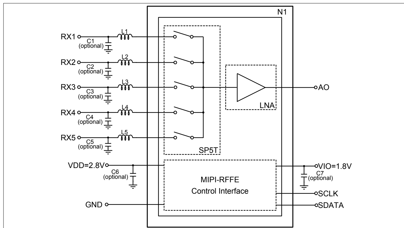
Figure 8: BGM15HA12 Application Schematic
