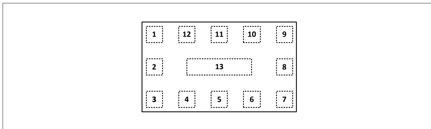
Figure 7: BGM15HA12 Pin Configuration (top view)
