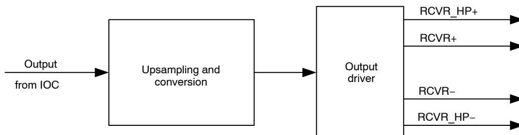
Figure 9. Output Stage
