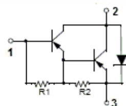
PIN 1. BASE 2. COLLECTOR 3. EMITTER TO-220C package
