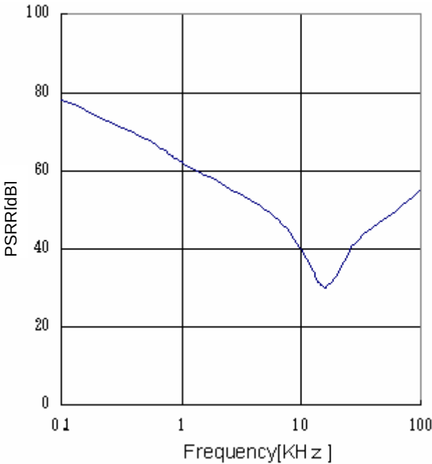
Fig.21 PSRR ( I_o=0mA )
