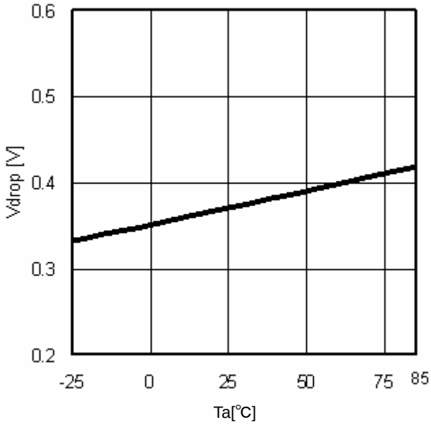
Fig.18 Minimum dropout Voltage1 ( V_{CC}=5V , I_O=-0.5A )
