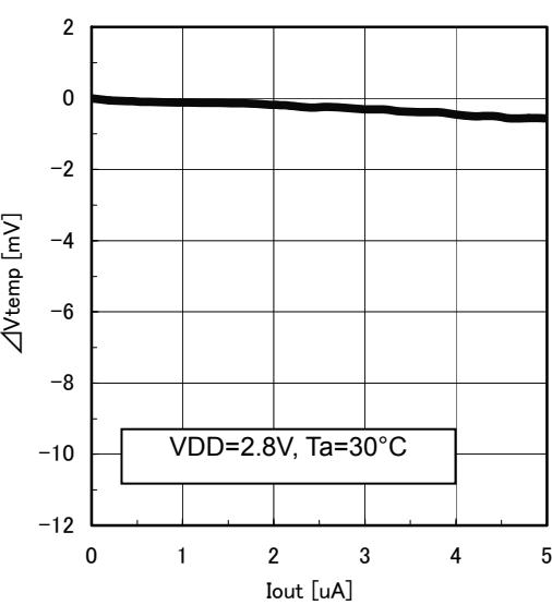
Fig4. Vtemp Voltage vs. Output Current
