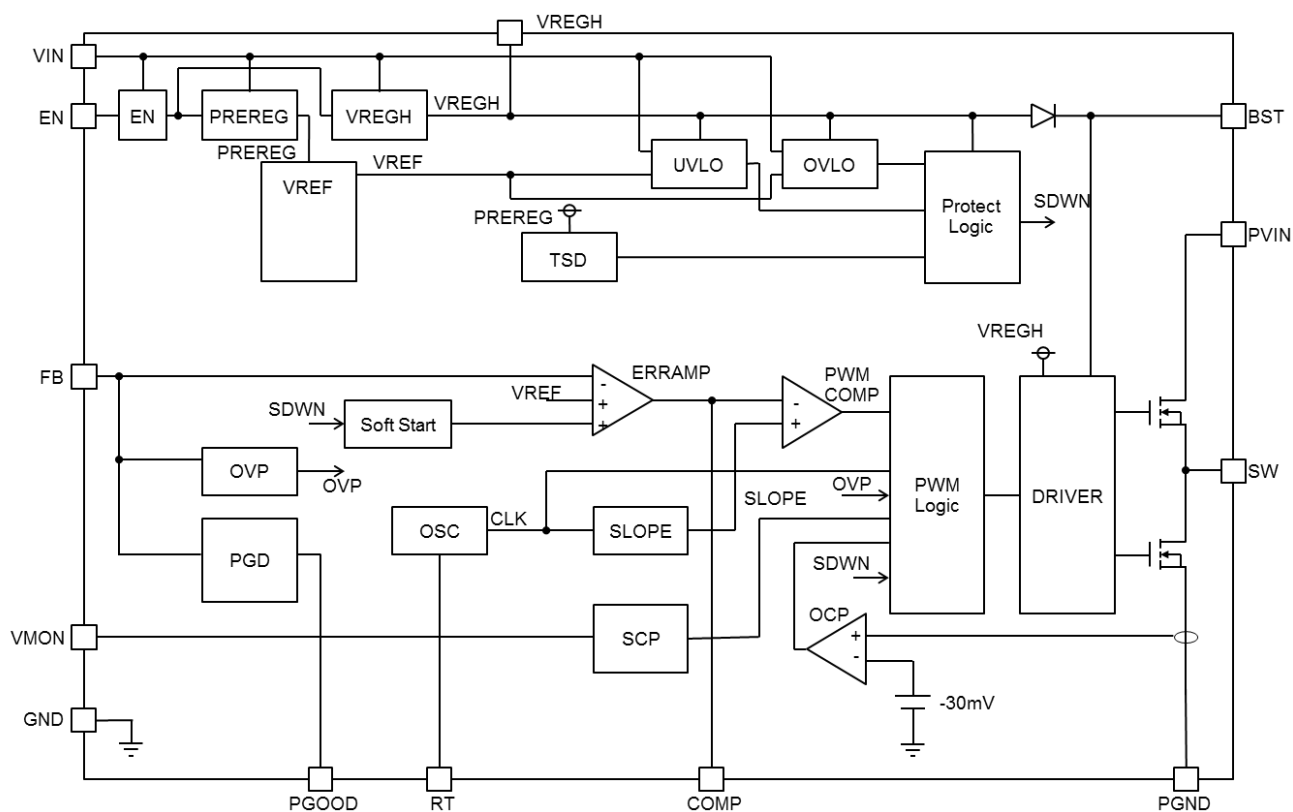
Figure 3. Block Diagram
