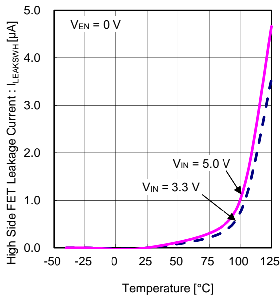
Figure 9. High Side FET Leakage Current vs Temperature
