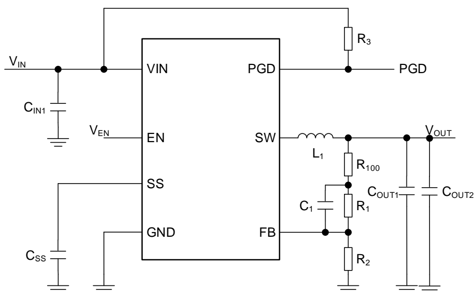
Figure 30. Reference Circuit 1
