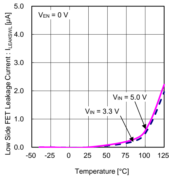
Figure 10. Low Side FET Leakage Current vs Temperature
