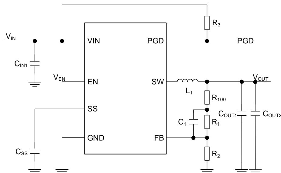
Figure 25. Application Circuit
