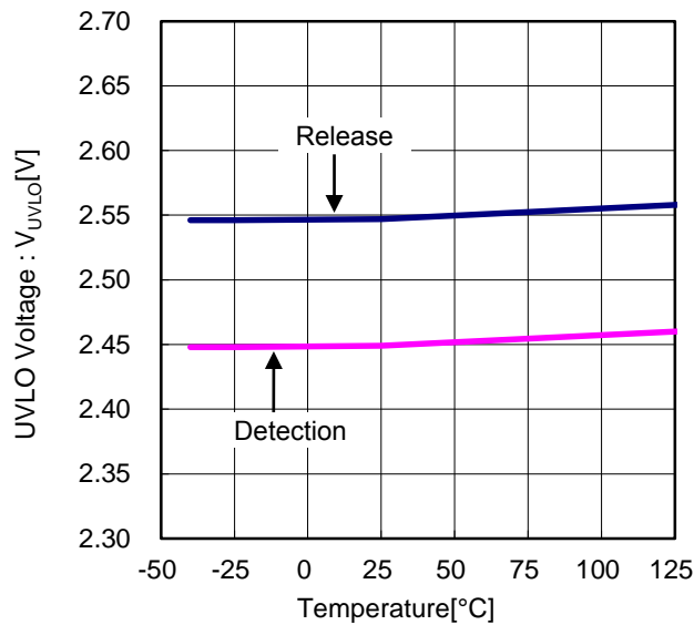
Figure 13. UVLO Voltage vs Temperature
