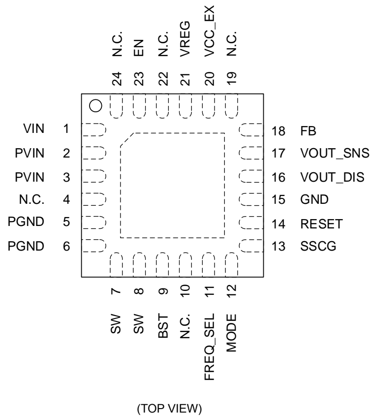
Figure 3. Pin Configuration
