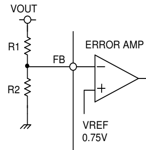
Figure 42. Output Voltage
