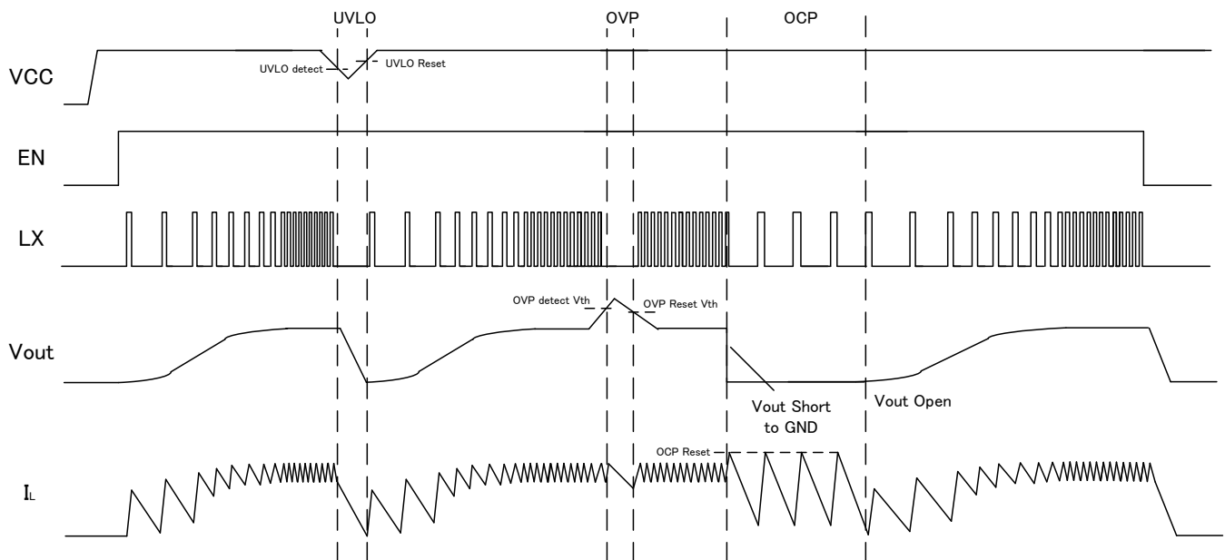
Figure 4. Timing Chart
