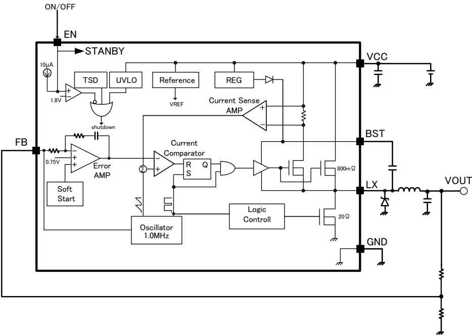
Figure 3. Block Diagram
