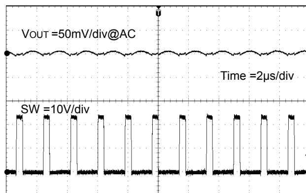
Figure 42. V_{OUT} Ripple ( V_{IN}=24V , V_{OUT}=5V , R_3=10k\Omega )
