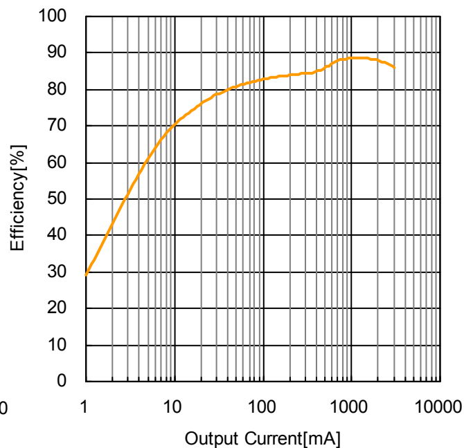
Figure 49. Efficiency - Output Current ( V_{IN}=24V , V_{OUT}=5.0V , R_3=15k\Omega , C_1=18pF )
