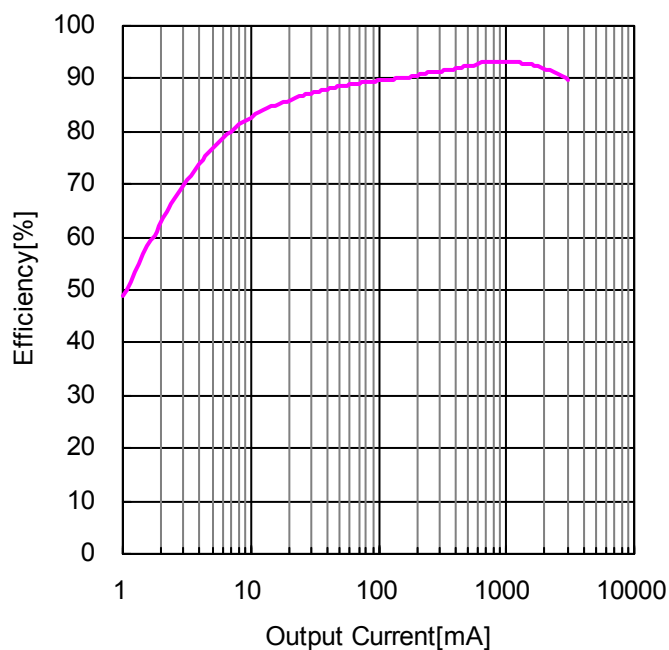
Figure 48. Efficiency - Output Current ( V_{IN}=12V , V_{OUT}=5.0V , R_3=15k\Omega , C_1=18pF )
