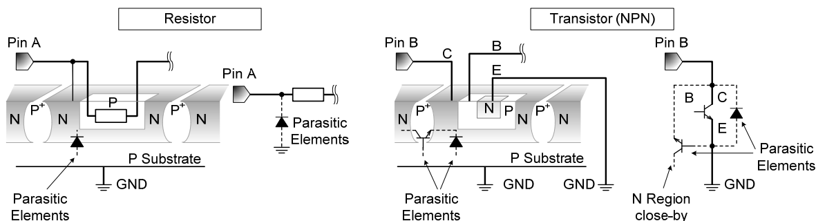
Figure 81. Example of monolithic IC structure
