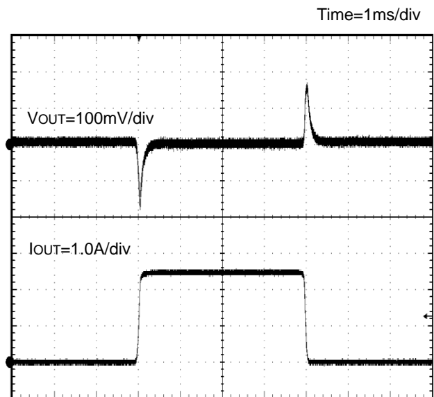
Figure 40. Load Transient Response IOUT=0A – 2.5A (VIN=24V, VOUT=5.0V, COUT=Ceramic22 \mu F \times 2)
