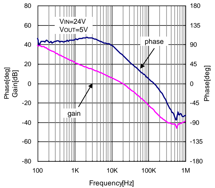
Figure 38. Loop Response (VIN=24V, VOUT=5V, IOUT=2.5A, COUT=Ceramic22 \mu F \times 2)
