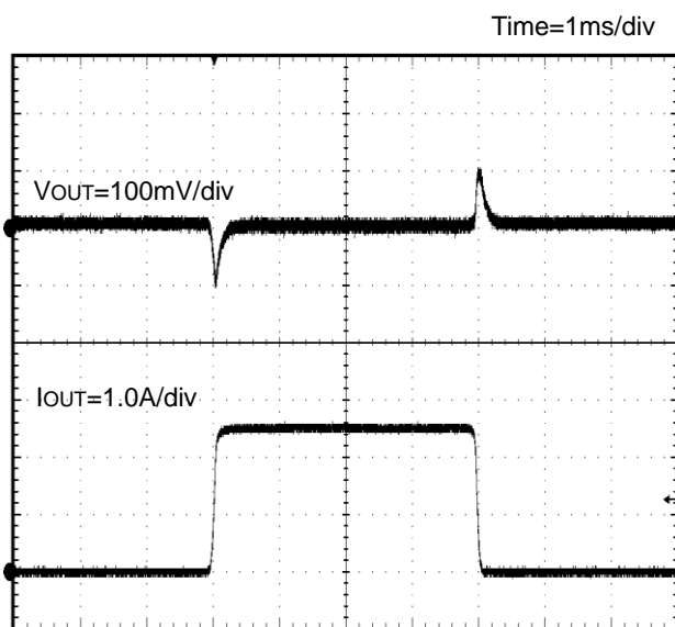
Figure 39. Load Transient Response IOUT=0A – 2.5A (VIN=12V, VOUT=3.3V, COUT=Ceramic22 \mu F \times 2)
