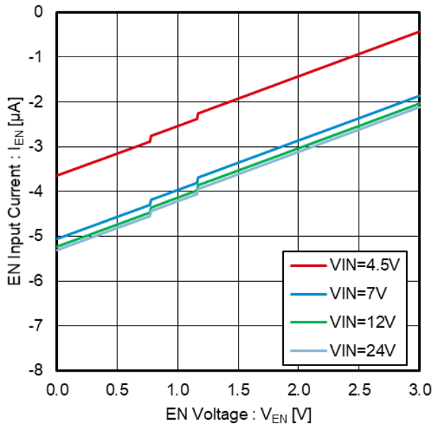
Figure 5. EN Input Current vs EN Voltage
