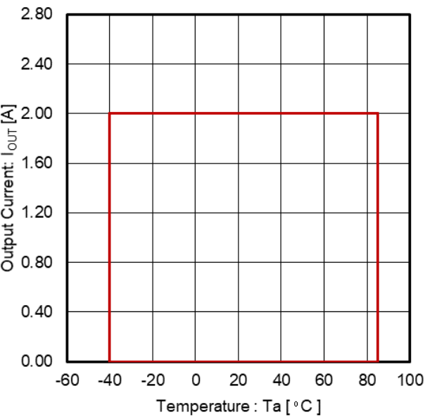
Figure 29. Output Current vs Temperature (Note 1) Operating Range: Tj < 150 °C (VIN = 24 V, VOUT = 12 V)
