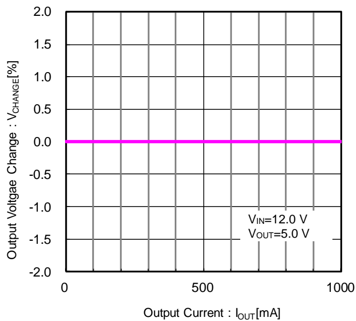
Figure 20. V_{OUT} Load Regulation
