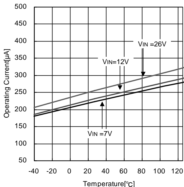
Figure 4. Operating Current - Temperature
