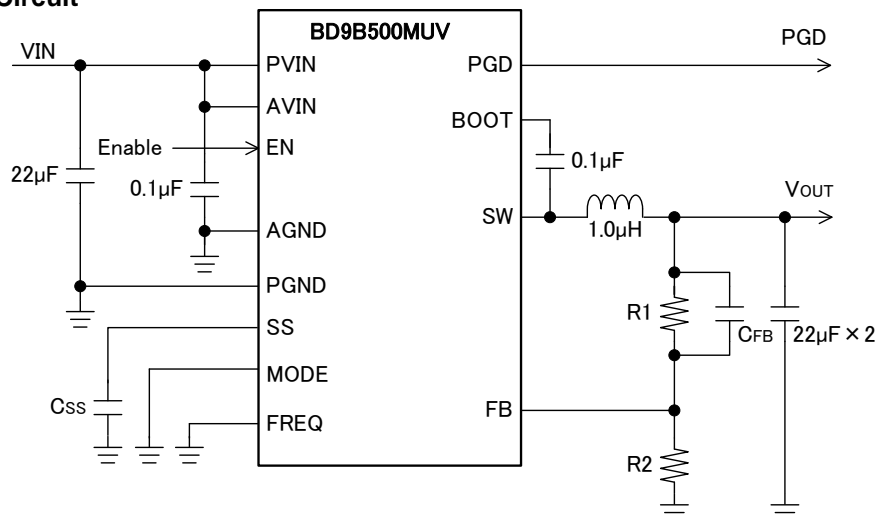
Figure 1. Application Circuit
