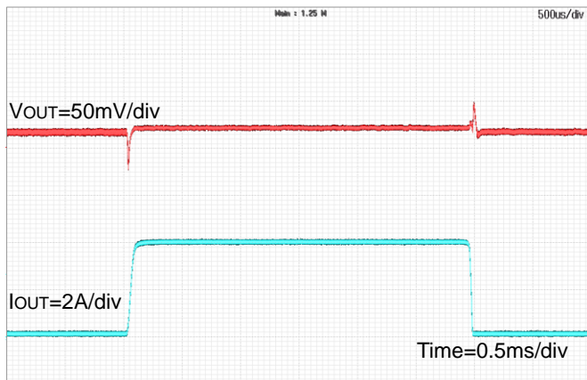
Figure 38. Load Transient Response I_{OUT}=0.1A to 4A ( V_{IN}=5V , V_{OUT}=1.2V , FREQ=L , MODE=L , C_{OUT}=Ceramic\ 44\mu F )
