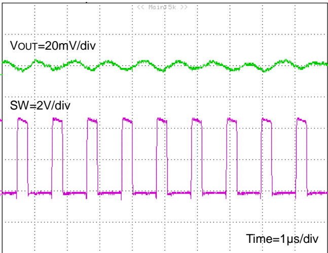
Figure 35. Switching Waveform ( V_{IN}=5\text{V} , V_{OUT}=1.2\text{V} , \text{FREQ}=\text{H} , I_{OUT}=5\text{A} )
