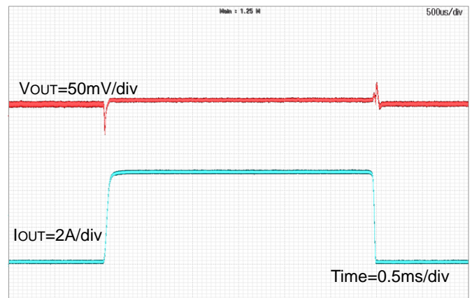
Figure 39. Load Transient Response I_{OUT}=0.1A to 5A ( V_{IN}=5V , V_{OUT}=1.2V , FREQ=L , MODE=H , C_{OUT}=Ceramic\ 44\mu F )
