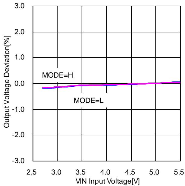
Figure 36. Line Regulation ( V_{OUT}=1.2V , L=1.0\mu H , FREQ=H , I_{OUT}=5A )
