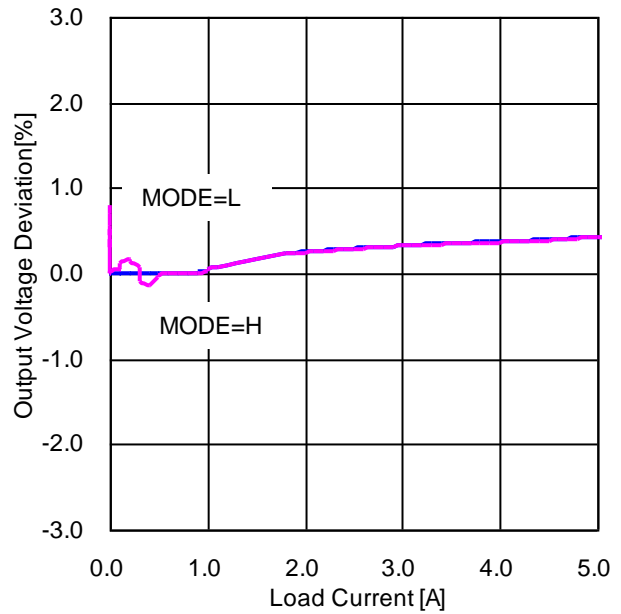
Figure 37. Load Regulation ( V_{IN}=5V , V_{OUT}=1.2V , L=1.0\mu H , FREQ=H )
