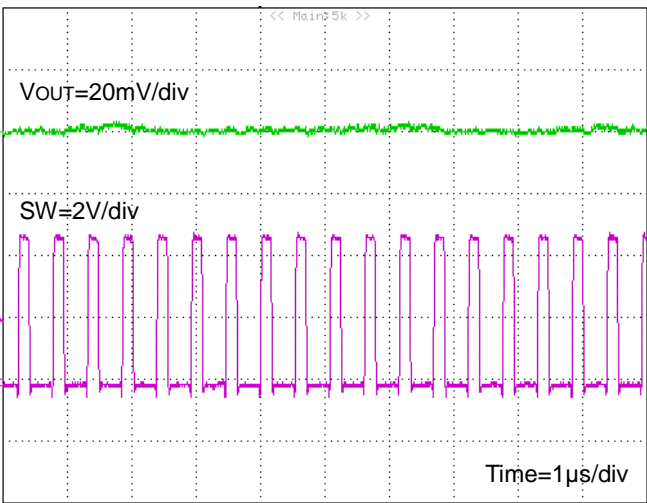
Figure 33. Switching Waveform ( V_{IN}=5\text{V} , V_{OUT}=1.2\text{V} , \text{FREQ}=\text{L} , I_{OUT}=5\text{A} )
