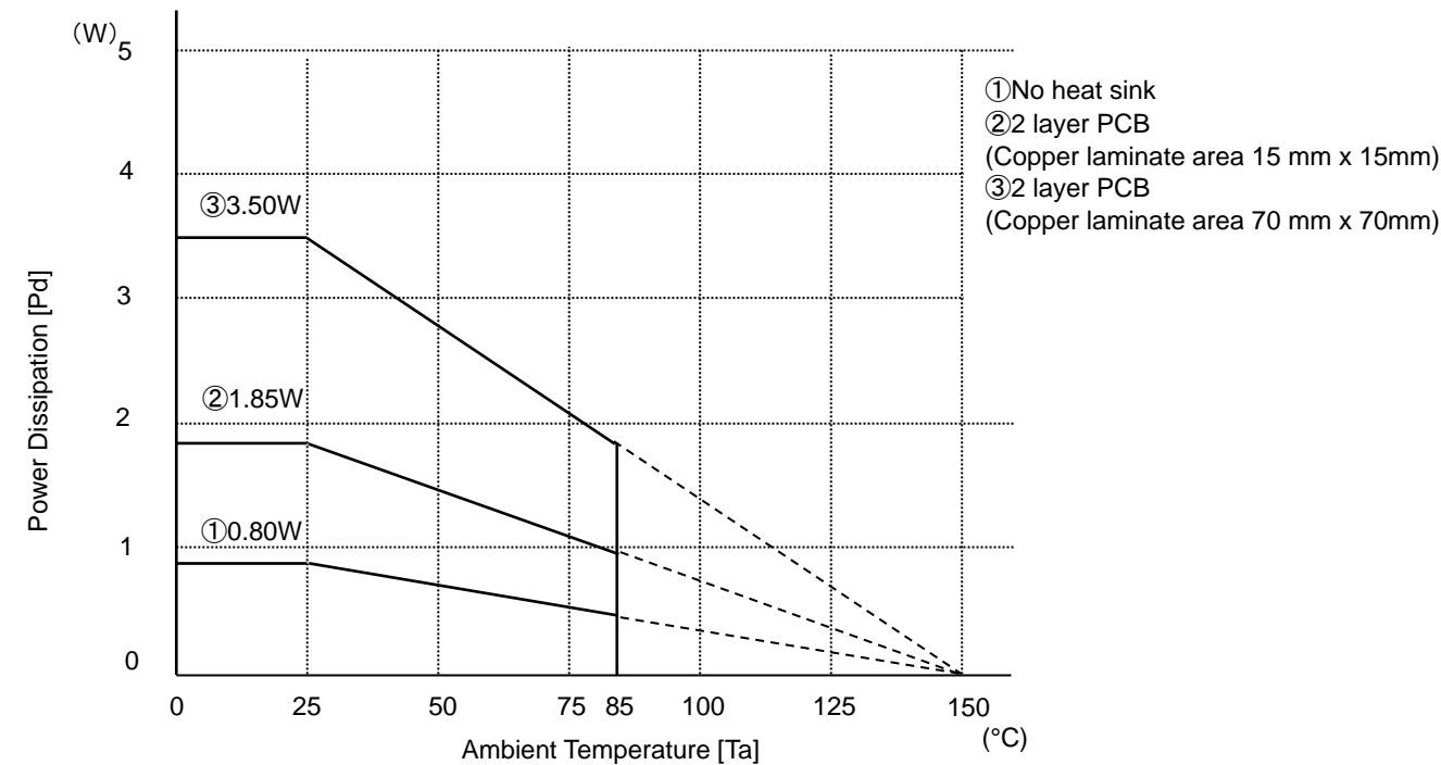
Figure 18. Power Dissipation
