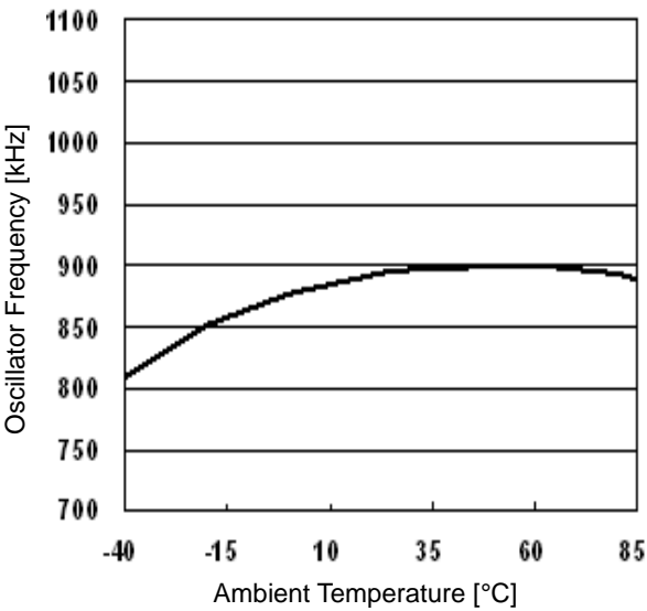
Figure 6. Oscillator Frequency vs Ambient Temperature
