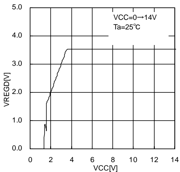
Figure.16 VREGD- VCC
