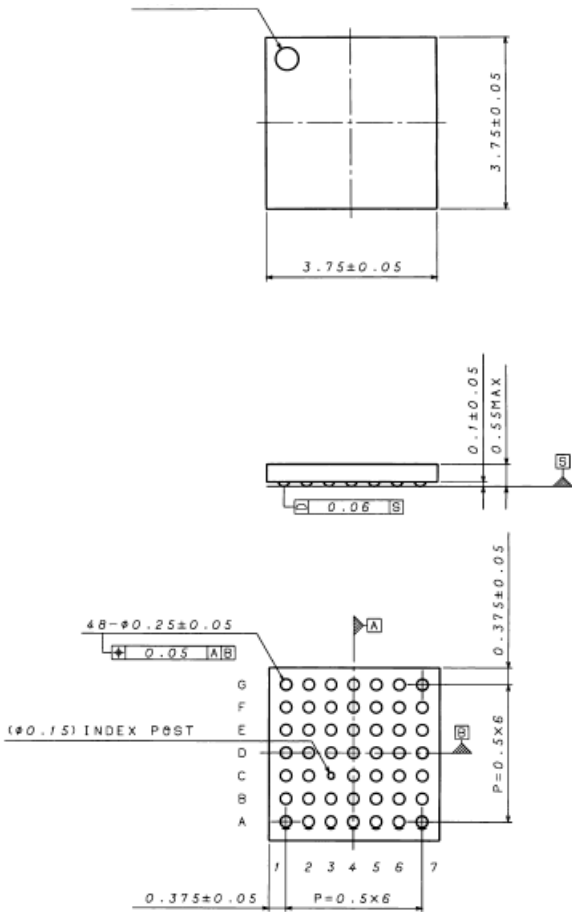
Figure. 64 Package dimensions
