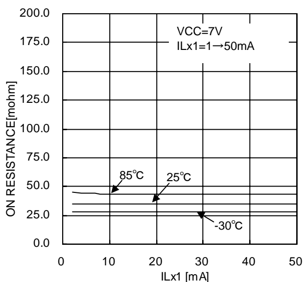
Figure.35 Lx1 Low side FET RON (Ta=-30°C, 25°C, 85°C)
