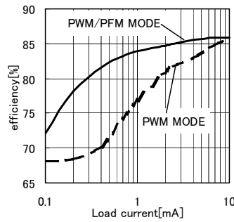
Fig.2 CH2 Current Load to Efficiency ( V_{IN2A}=3.5\text{V} , V_{IN2B}=10\text{V} , V_{o2}=12\text{V} )
