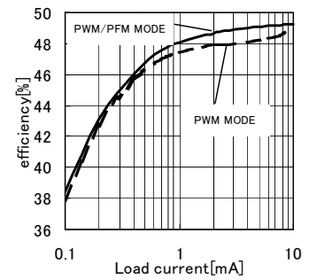
Fig.3 CH3 Current Load to Efficiency ( V_{IN3}=10\text{V} , V_{o3}=-5\text{V} )
