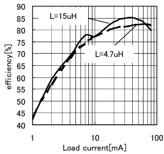
Fig.1 CH1 Current Load to Efficiency ( V_{o1}=10\text{V} )
