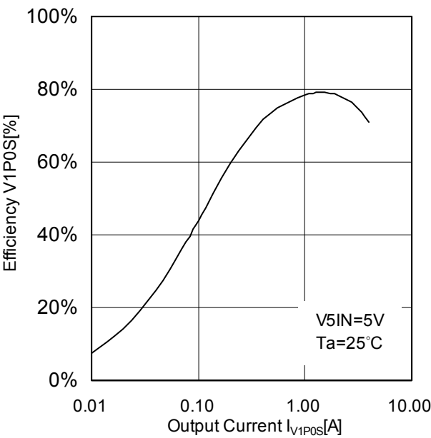
Figure 49. Efficiency V1P0S vs Output Current I_{V1P0S}
