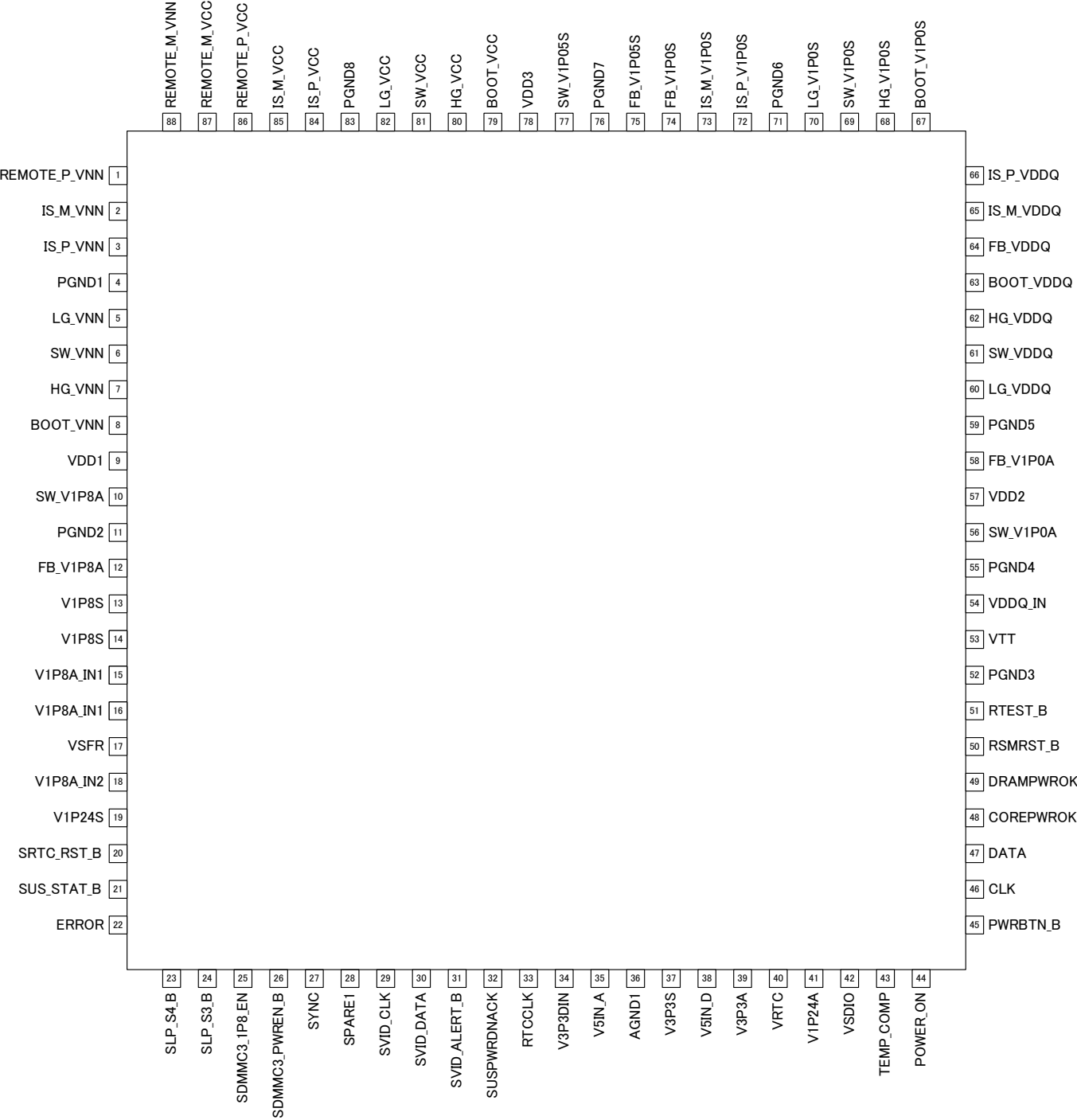
Figure 2. Pin Configuration
