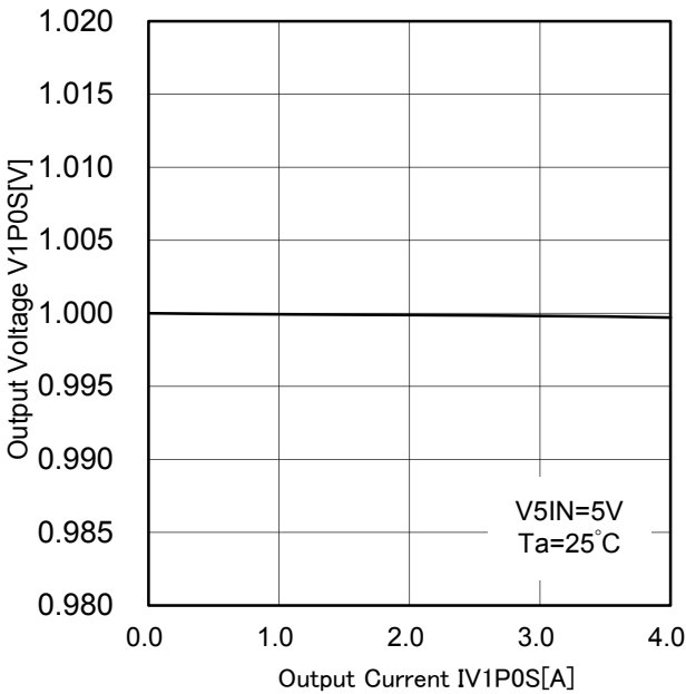
Figure 26. Output Voltage V1P0S vs Output Current I_{V1P0S}
