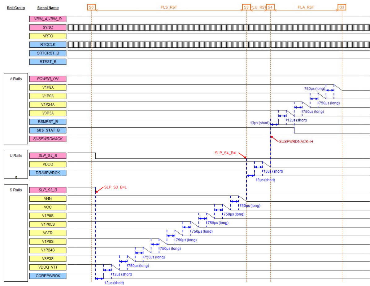
Figure 67. Cold Off Timing Chart
