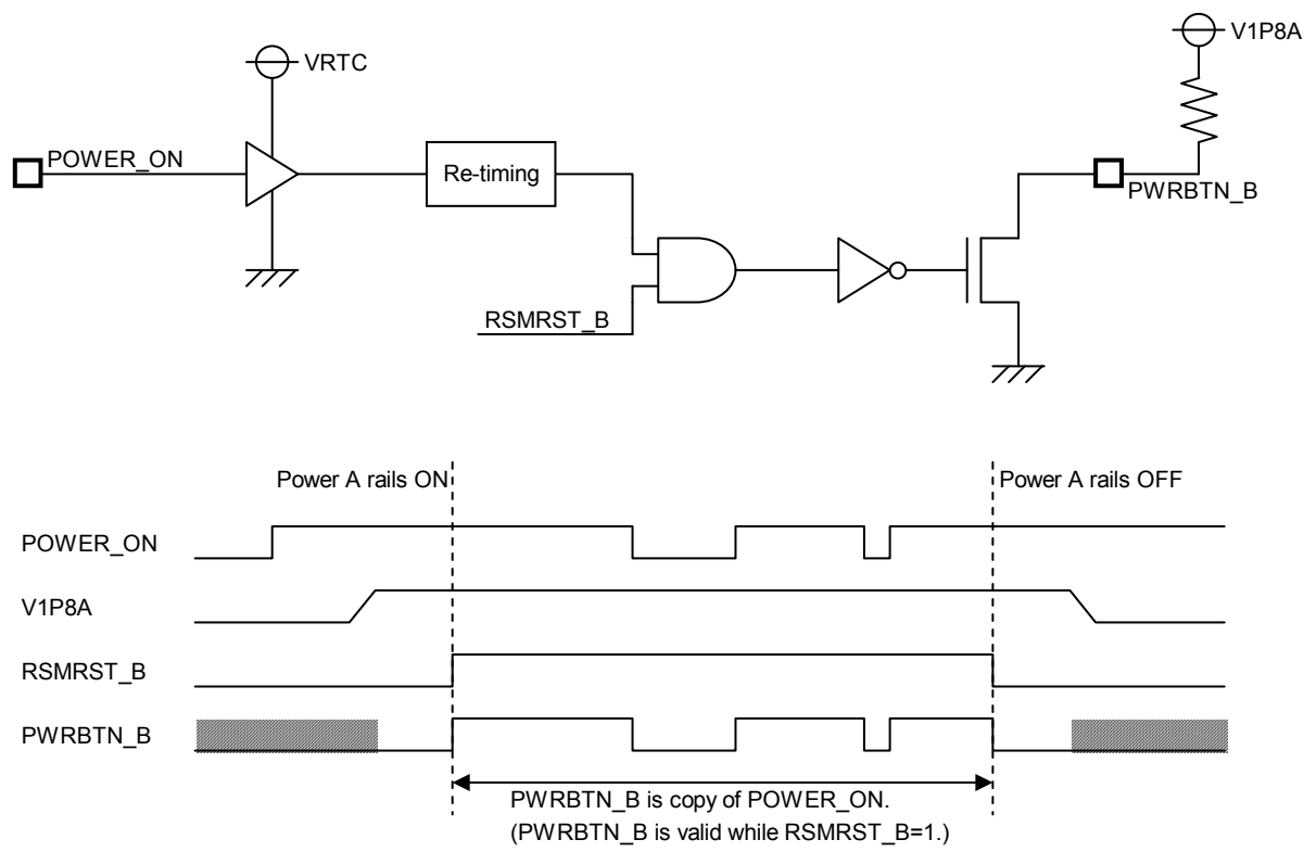
Figure 72. PWRBTN_B Timing Chart
