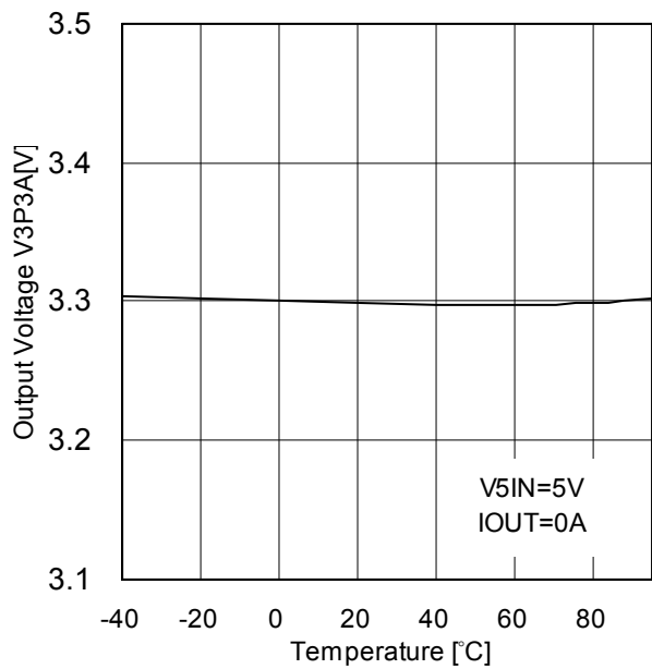
Figure 29. Output Voltage V3P3A vs Temperature
