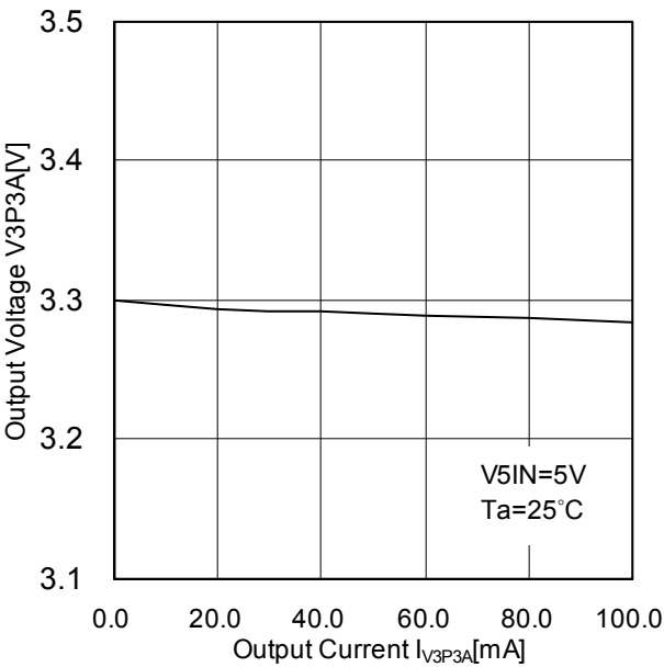
Figure 12. Output Voltage V_{3P3A} vs Output Current I_{V3P3A}
