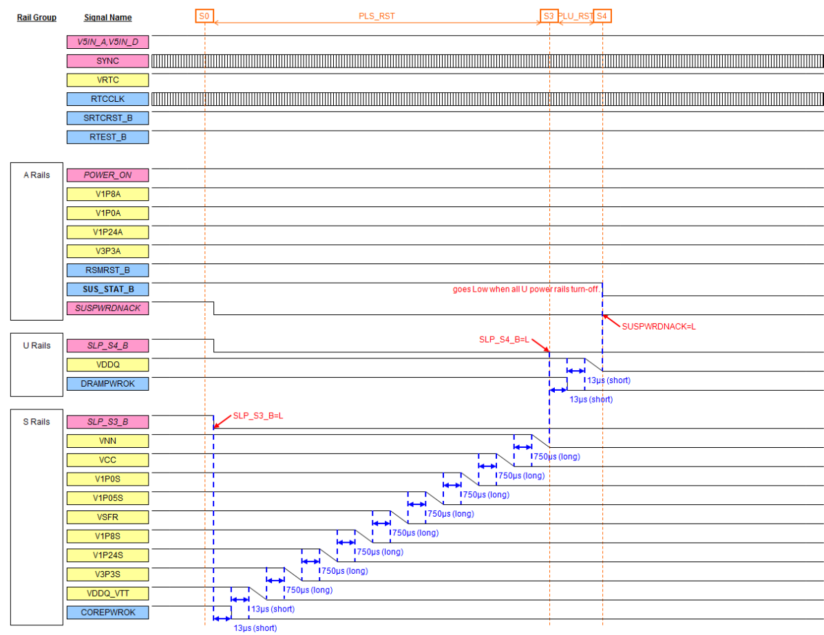
Figure 68. Enter SOC S4 Timing Chart
