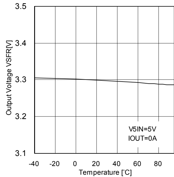
Figure 28. Output Voltage VSFR vs Temperature
