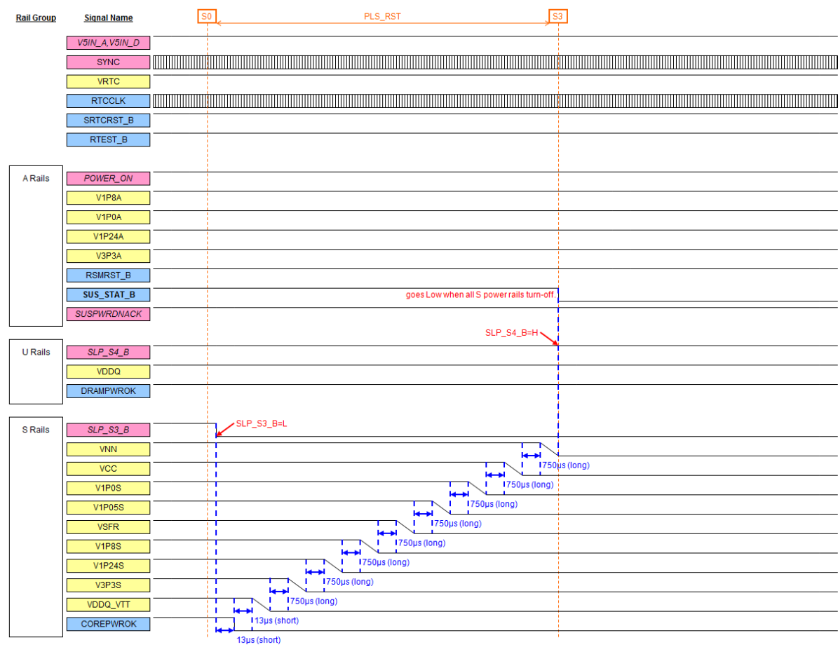
Figure 70. Enter SOC S3 Timing Chart
