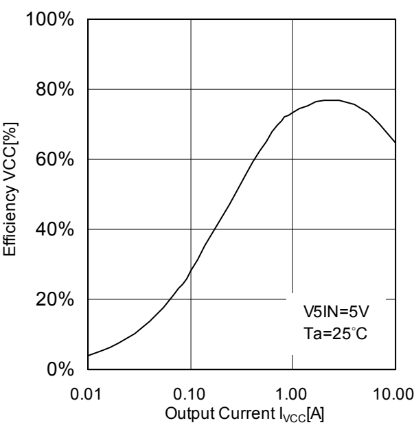
Figure 47. Efficiency VCC vs Output Current I_{VCC}
