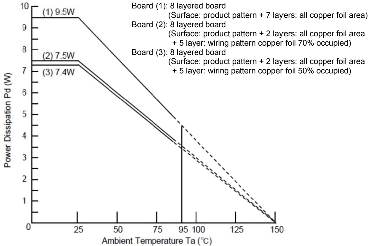
Figure 76. Power Dissipation
