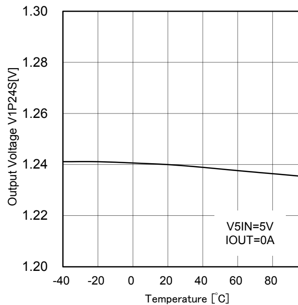
Figure 37. Output Voltage V1P24S vs Temperature
