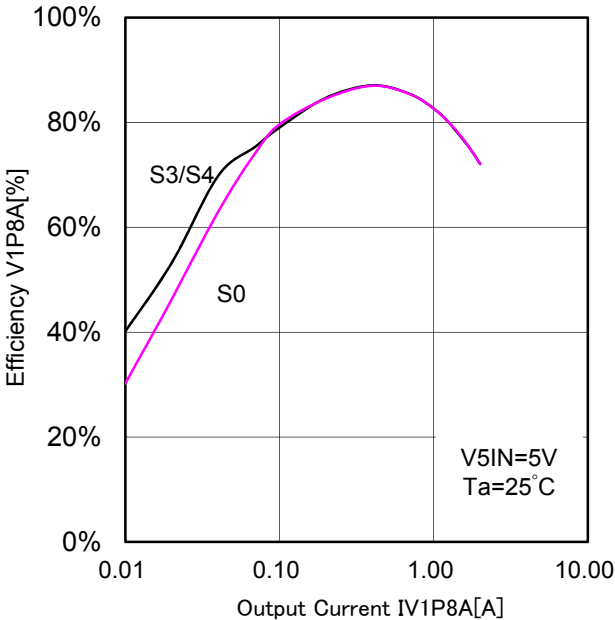
Figure 45. Efficiency V1P8A vs Output Current I_{V1P8A}
