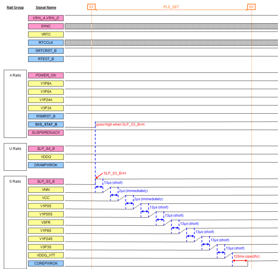
Figure 71. Exit SOC S3 Timing Chart
