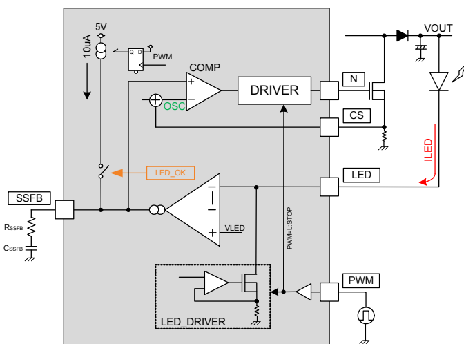
Figure 12. Circuit behavior at startup
