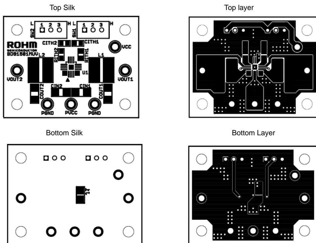
Figure.39 Layout Diagram
