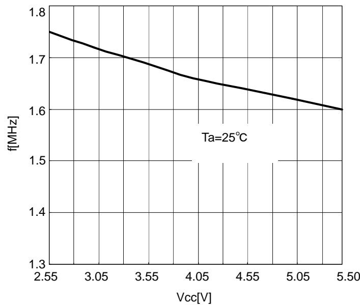
Figure.11 VCC-Fosc
