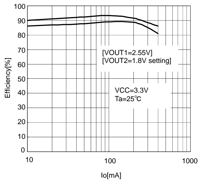
Figure.9 Efficiency
