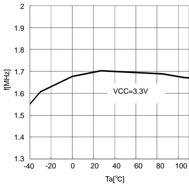
Figure.10 Ta-Fosc
