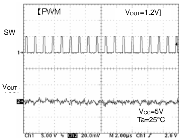
Figure 16. SW Waveform ( I_o=10\text{mA} )
