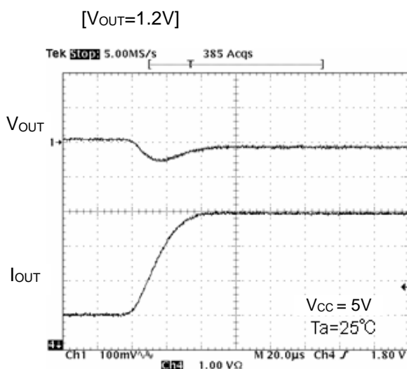
Figure 17. Transient Response (I O =1A to 4A, 20μs)
