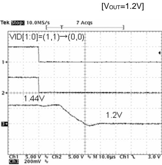
Figure 20. Change Response
