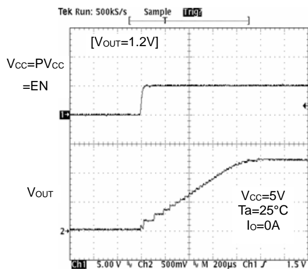
Figure 14. Soft-Start Waveform
