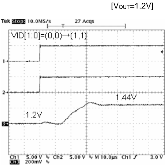
Figure 19. Change Response
