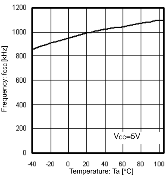
Figure 9. Frequency vs Temperature
